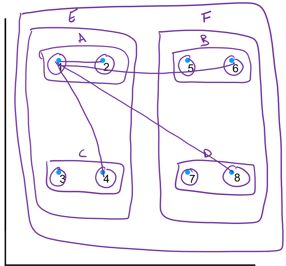
Complete Link clustering (Farthest pair)
