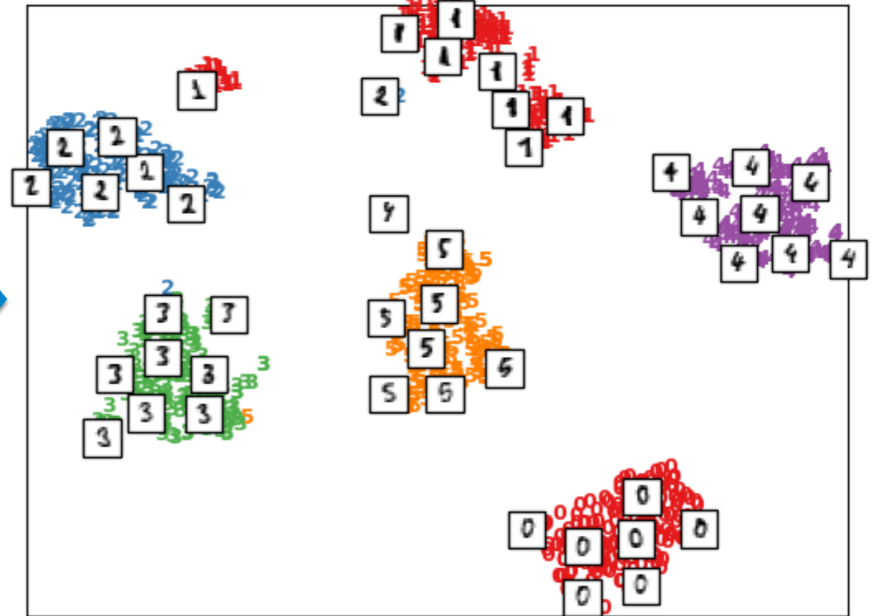
t-SNE embedding of the digits (time 5.26s)
